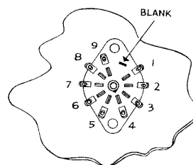
NUMBERING ON 9-PIN TUBE SOCKET
