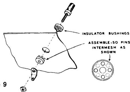
PILOT LIGHT ASSEMBLY
