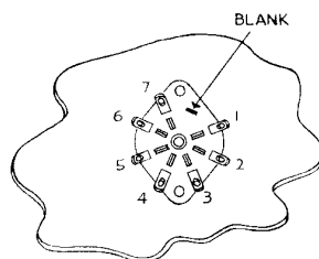
NUMBERING ON 7-PIN TUBE SOCKET
